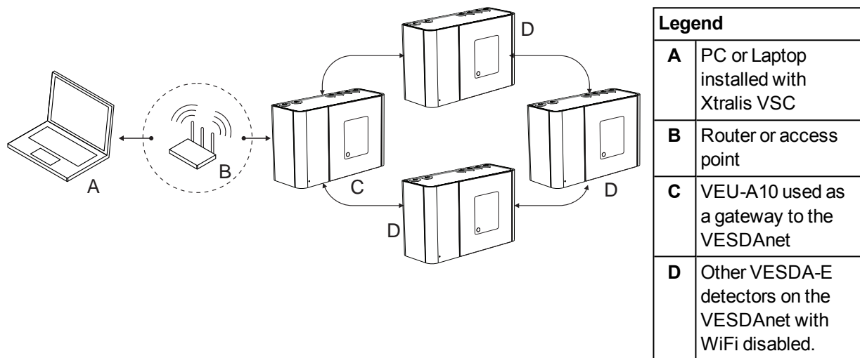
Figure 5-11: Connection to a detector via another detector on VESDAnet using a WiFi connection
