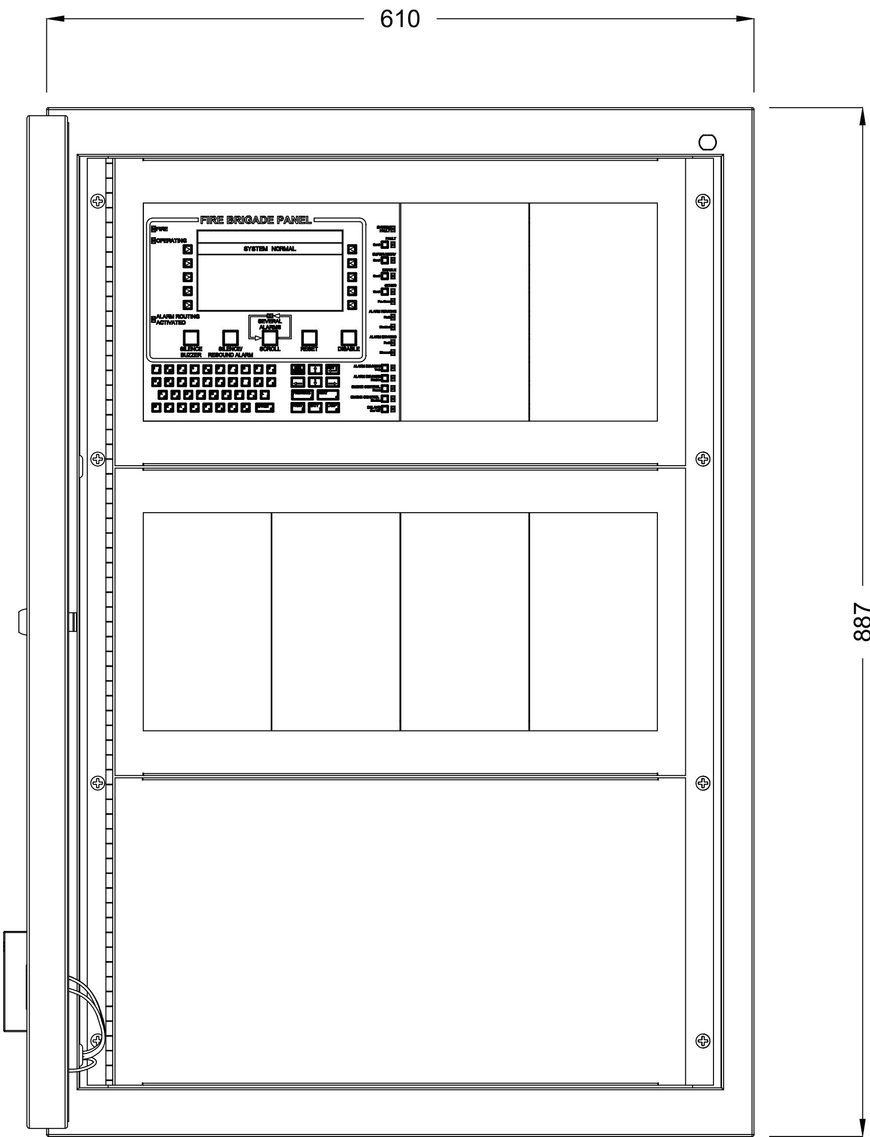
FRONT VIEW
