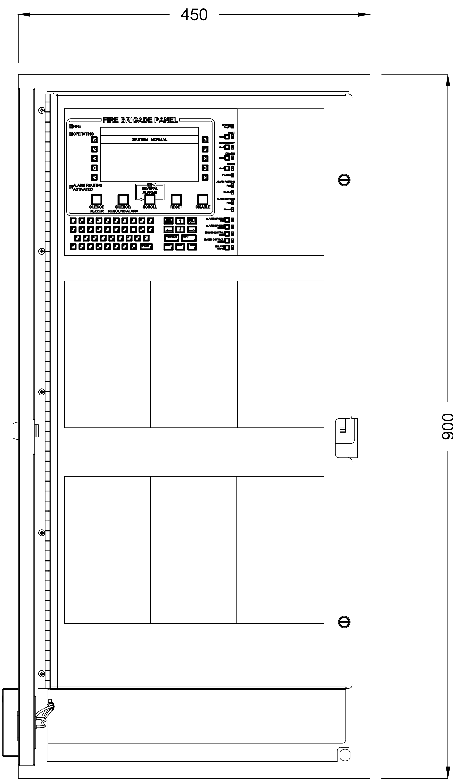
FRONT VIEW
