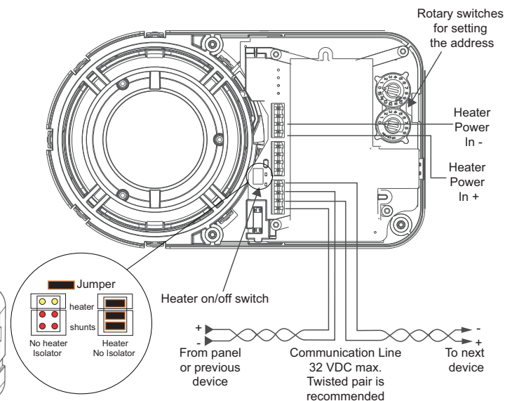
Figure 2-11: Wiring Diagram
