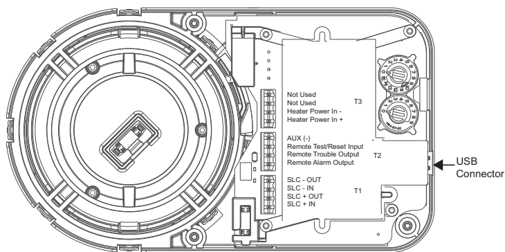
Figure 2-10: Wiring Connections at Detector
