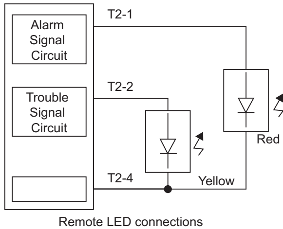
Figure 2-13: Wiring Diagram (Remote LEDs)
