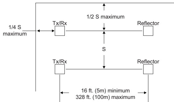
Figure 2-2: Smooth Ceiling (Top View)
