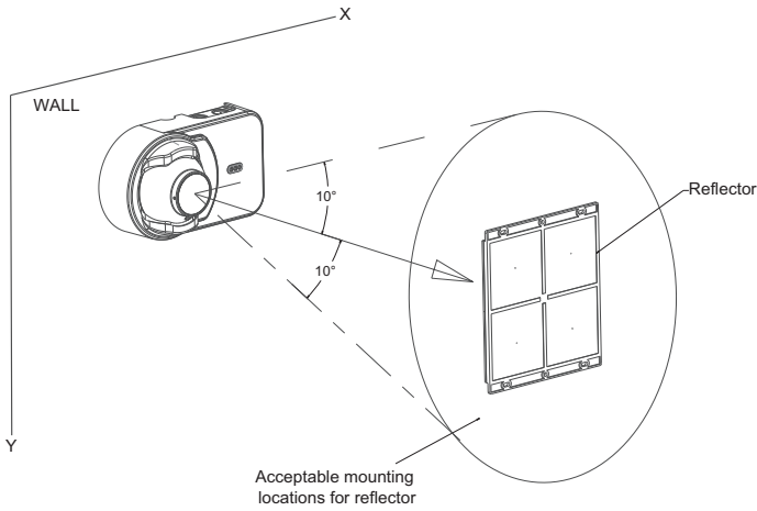
Figure 2-5: Reflector Mounting Guidelines
