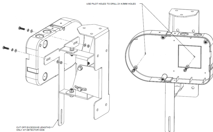
Figure 2-9: Detector Mounting Guidelines
