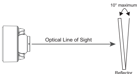
Figure 2-7: Reflector Mounting Guidelines
