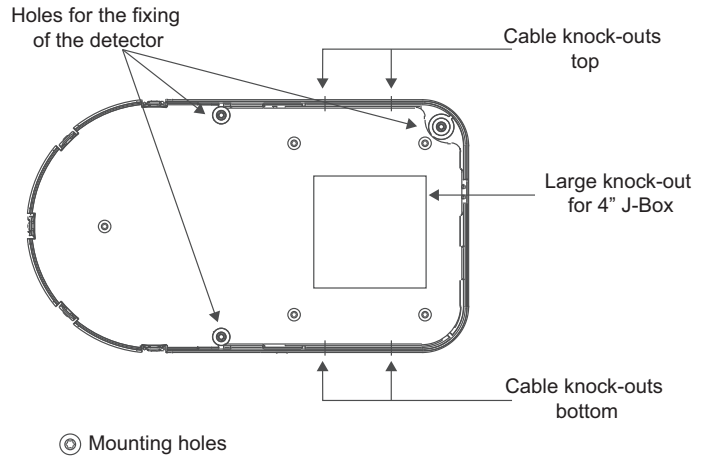
Figure 2-8: Mounting pilot holes
