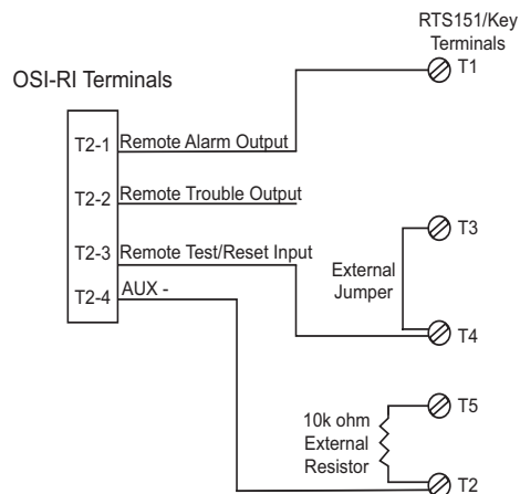
Figure 2-12: Wiring Diagram (RTS151)
