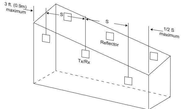
Figure 2-3: Sloped Ceiling (Shed Type)
