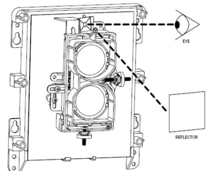
Figure 3: Coarse Alignment Procedure
