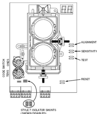
Figure 1: Switch Locations
