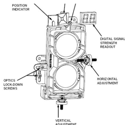
Figure 2: Alignment Adjustment Locations
